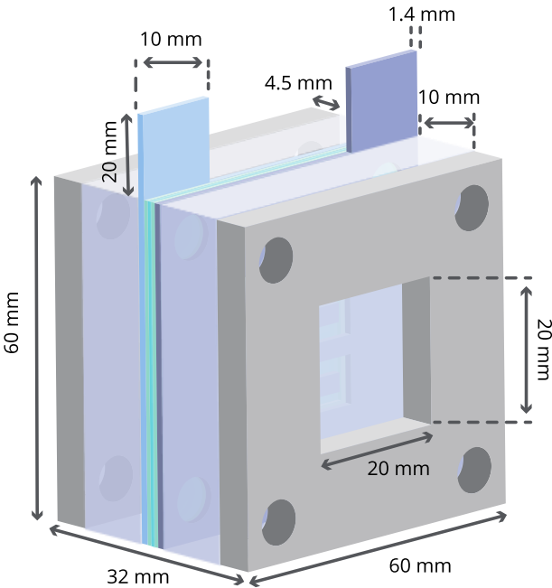
Visual membrane electrode assembly electrolyzer dimensions
